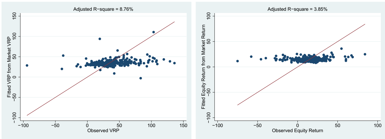
Fig. 3. Fitted VRPs/equity returns vs. observed VRPs/equity returns. This figure plots fitted VRPs (equity returns) versus observed VRPs (equity returns). The fitted VRP (equity return) for firm i is estimated as VRP_i = \lambda_0^{VRP} + \lambda_1^{VRP} \times \beta_i^{VRP} ( R_i = \lambda_0^{CAPM} + \lambda_1^{CAPM} \times \beta_i^{CAPM} ), where the \lambda 's and \beta 's are estimated using the standard two-stage regressions of testing CAPM. In the first stage, time-series regressions for each firm i to estimate its \beta_i^{VRP} and \beta_i^{CAPM} , respectively: VRP_{it} = \alpha_i^{VRP} + \beta_i^{VRP} \times VRP_{MKT} + \epsilon_{it}^{VRP} for VRP and R_{it} = \alpha_i^{CAPM} + \beta_i^{CAPM} \times R_{MKT} + \epsilon_{it}^{CAPM} for CAPM. Then each firm's average VRP, \overline{VRP}_i , and average equity return, \overline{R}_i , are computed respectively. The second-stage cross-sectional regressions are \overline{VRP}_i = \lambda_0^{VRP} + \lambda_1^{VRP} \times \beta_i^{VRP} + u_i^{VRP} for VRP and \overline{R}_i = \lambda_0^{CAPM} + \lambda_1^{CAPM} \times \beta_i^{CAPM} + u_i^R for CAPM.
