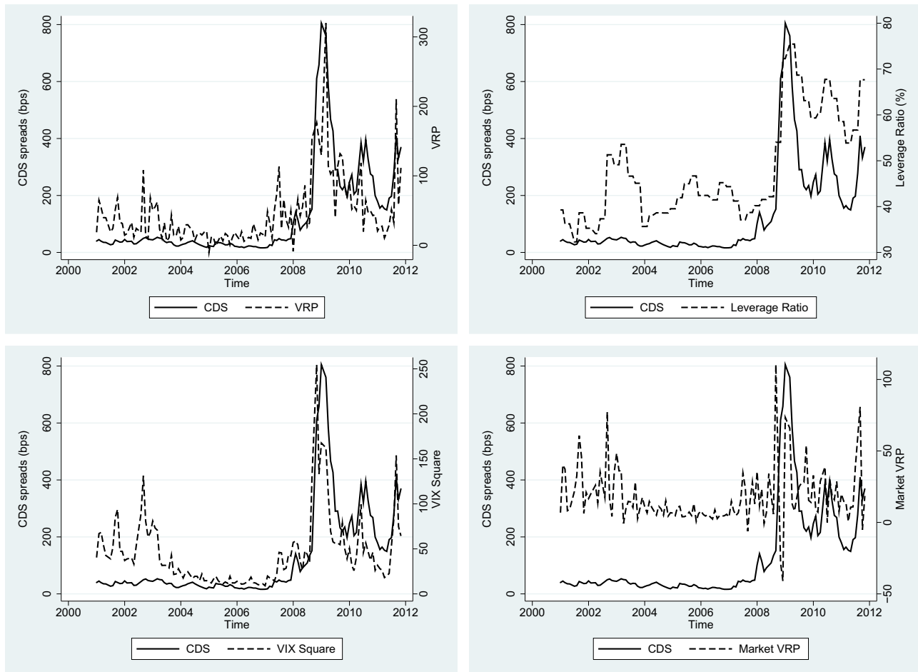
Fig. 2. Time series of CDS spreads, VRP, leverage ratio, MVRP and VIX for General Motor Ltd. This figure illustrates the dynamic relationships between CDS spreads and VRP, market VRP, VIX and leverage ratio for a representative firm in our sample: ALCOA.
